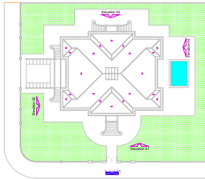
Roof Plan
