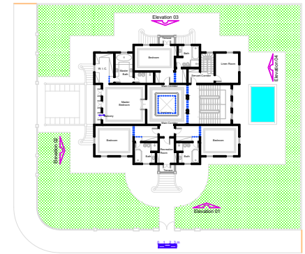
Second Floor Plan A = 260,89 m 2
