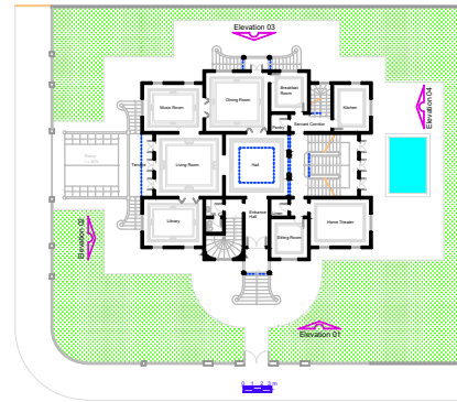
First Floor Plan A = 260,38 m 2
