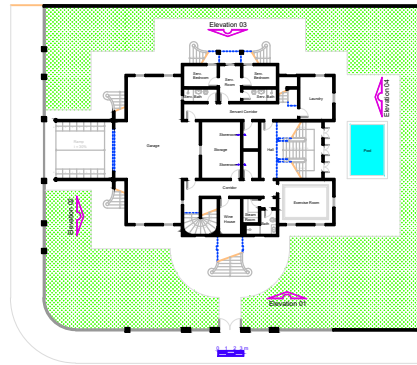
Lower Floor Plan A = 287,22 m 2
